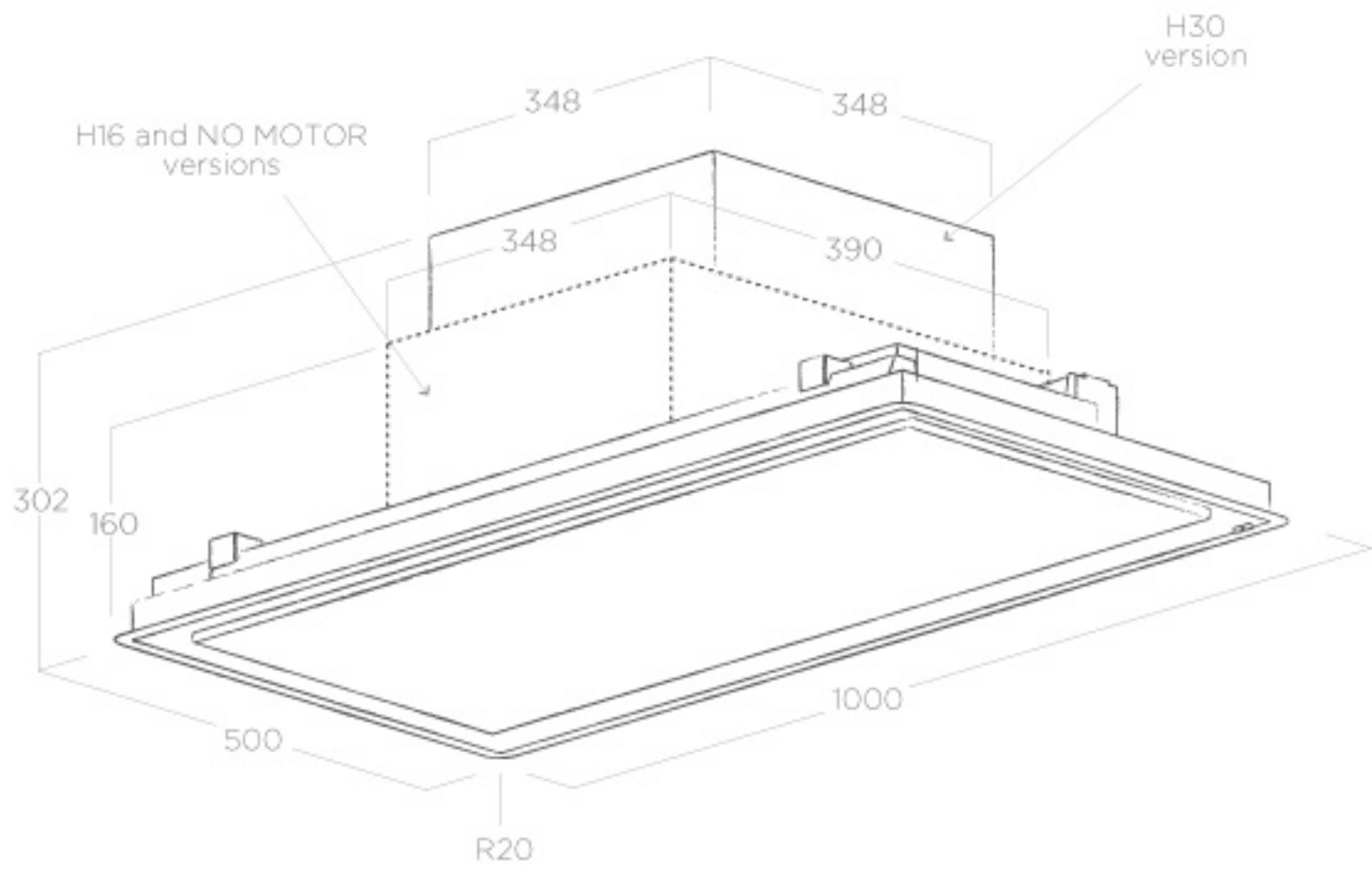
FALSE CEILING CUT: 480X980
